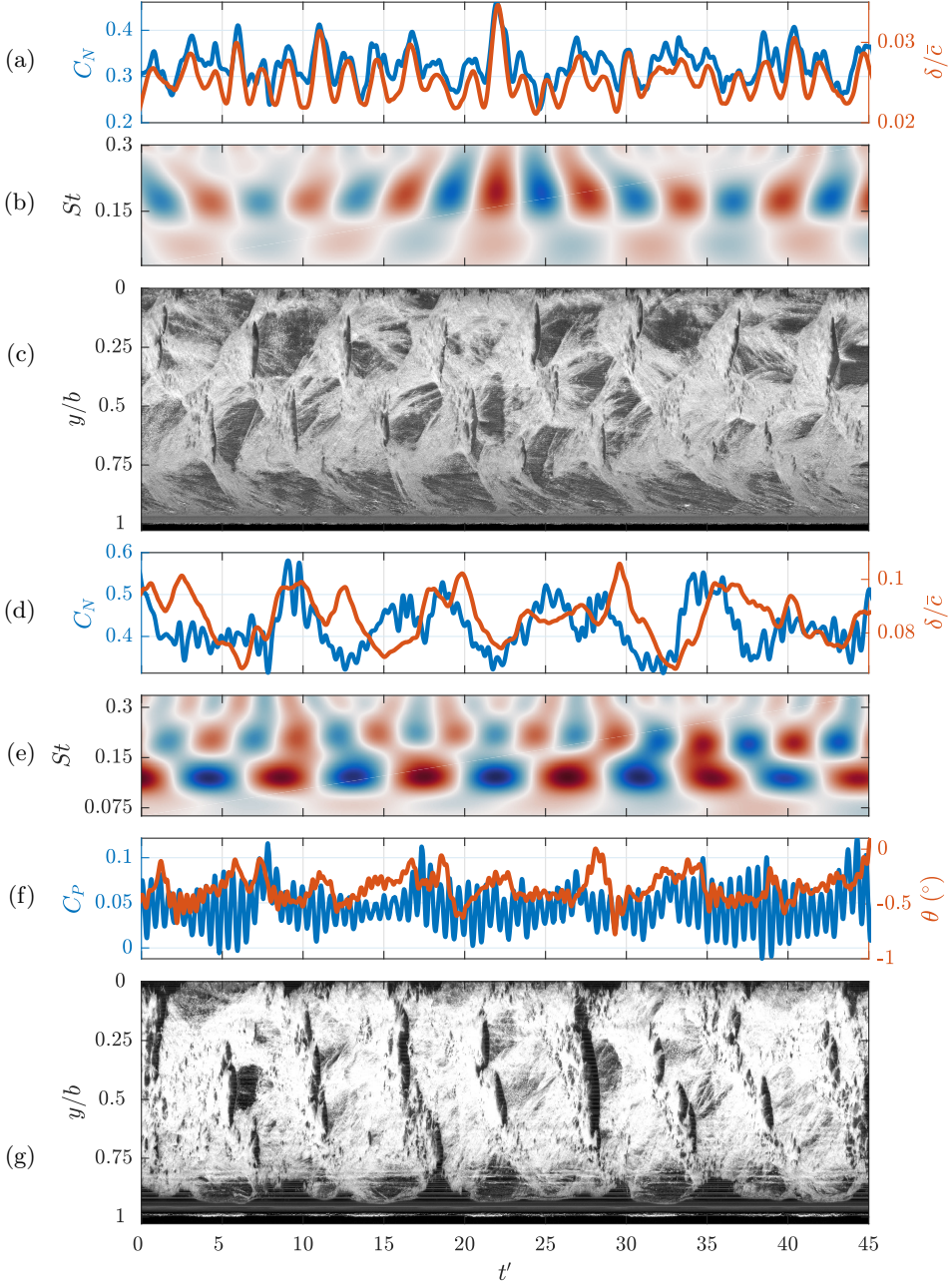
FIGURE 24. Synchronised time series of the normal force ( C_N ) and tip displacement ( \delta/\bar{c} ) (a (stiff), d(flexible)) along with the flexible hydrofoils pitching moment and twist ( \theta ) (f) at \sigma = 0.4 and 0.5 for the stiff and flexible hydrofoil, respectively. The real value of the Morlet wavelet transforms for C_N (b(stiff), e(flexible)) shows the different dominant modes of either hydrofoil, also evident in the space-time plots for the stiff (c) and flexible (g) hydrofoils both taken at x/c_{\text{root}} = 0.5 .
