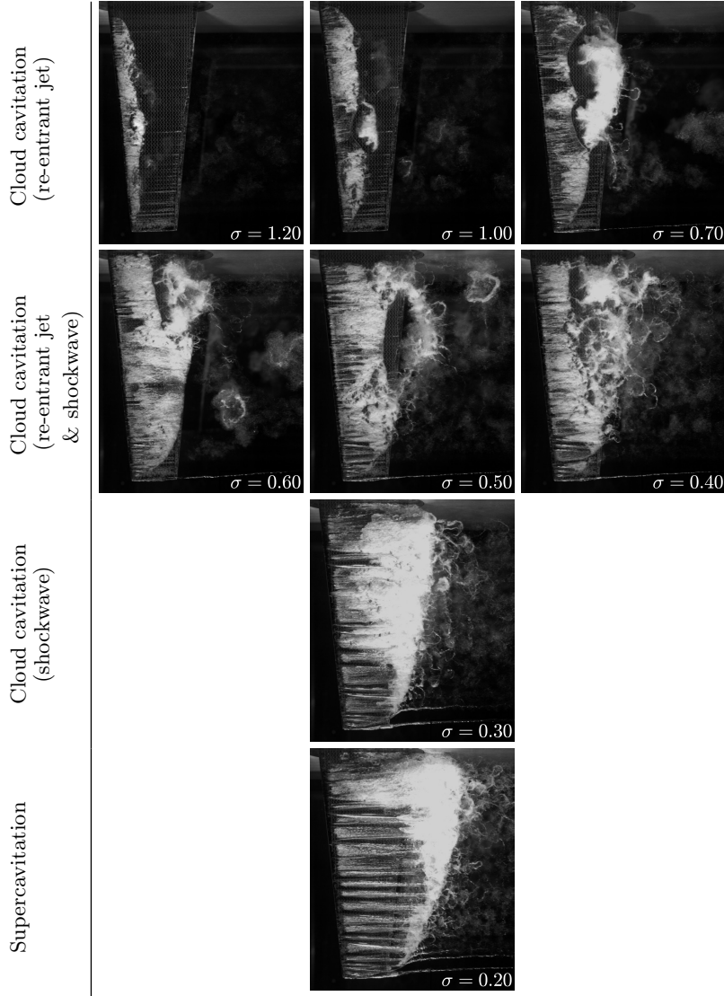
FIGURE 7. Images of the flexible hydrofoil experiencing the differing cavitation regimes through the range of \sigma below inception. The flexible hydrofoil first experiences re-entrant jet-driven cloud cavitation for the conditions tested, not experiencing stable sheet cavitation as observed on the stiff hydrofoil for \sigma \geq 1.1 . The attached cavity and re-entrant jet-driven cloud cavitation develops further as \sigma is reduced ( 0.65 \leq \sigma \leq 1.2 ). A further reduction in \sigma , with cavity length extending to the trailing edge, upstream propagating condensation shockwaves develop, resulting in a complex coupled mechanism involving both the re-entrant jet and shockwave instabilities for 0.4 \leq \sigma \leq 0.6 . Once \sigma reaches 0.3, shedding is solely driven by shockwave propagation. Supercavitation is present for ( \sigma < 0.3 ) with a stable sheet cavity present over all the hydrofoil surface and the cavity break-up restricted to the cavity closure region downstream of the trailing edge. Supplementary material features high-speed movies that show the various shedding mechanisms.
