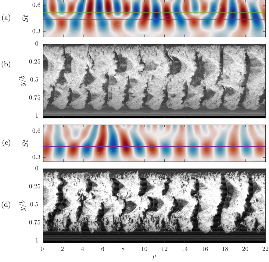
FIGURE 20. Both hydrofoils experience the formation of two shedding sites along the span at \sigma = 0.8 due to the spatial compatibility between the attached cavity and the planform geometry. This is shown by the spanwise space-time plots taken at x/c_{\text{root}} = 0.5 and 0.58 for the stiff (b) and flexible (d) hydrofoils, respectively. However, the real value C_N Morlet wavelet transform from the stiff hydrofoil (a) shows the multi-modal behaviour at St = 0.41 (purple horizontal line) and 0.50 (green horizontal line), while for the flexible hydrofoil (c), only the St = 0.40 (purple horizontal line) Type IIa mode is evident in the wavelet transform. Closer inspection of the cavitation behaviour towards the tip shows a higher degree of break-up on the flexible hydrofoil compared to the stiff, linked to the larger deformations.
