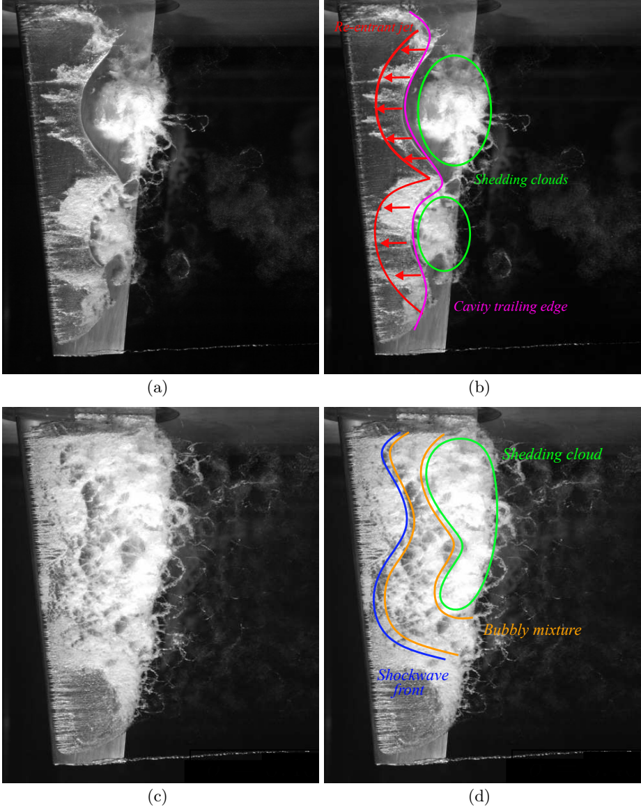
FIGURE 6. Typical example images of cloud cavitation due to re-entrant jet formation at \sigma = 0.7 (a) and shockwave formation at \sigma = 0.4 (c). In the annotated version of re-entrant jet-driven shedding (b), flow over the attached cavity reaches the cavity trailing edge (purple), where it impacts the hydrofoil surface, forming a re-entrant jet (red) underneath the cavity, eventually causing it to break-off and form shed clouds (green). In the annotated version of shockwave-driven shedding (d), collapse of the large attached cavity occurs first in the high pressure region downstream, causing a condensation shockwave (blue) to propagate upstream, breaking up the attached cavity into a bubbly mixture (orange) which forms a shedding cloud (green).
