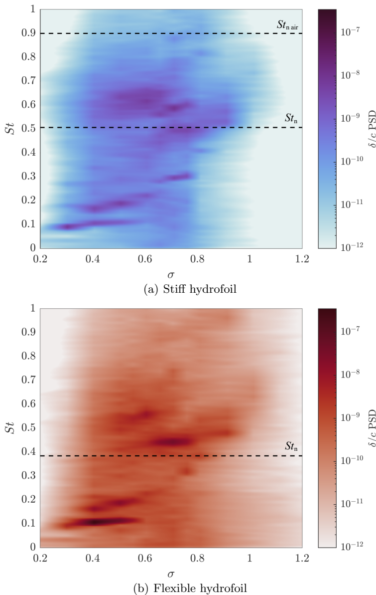
FIGURE 12. Spectrograms of \delta/\bar{c} for a range of \sigma showing the global unsteady behaviour of the bending deformations. Comparison of the stiff (a) and flexible (b) hydrofoils highlights the increased power of structural deformations on the flexible hydrofoil. This causes increased FSI, particularly at points of lock-in. Both hydrofoils exhibit similar trends observed in the C_N spectrograms with strong interactions with structural modes where the fully wetted natural frequency of the hydrofoils, shown non-dimensionally, St_n , as a horizontal dashed line.
