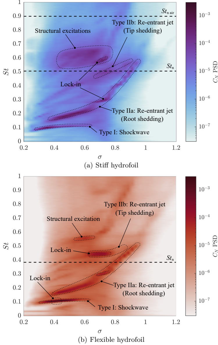
FIGURE 11. Spectrograms of C_N for a range of \sigma showing the global unsteady behaviour of the normal force. The results highlight the shockwave-driven Type I shedding frequency is predominately independent of \sigma while the re-entrant jet-driven Type IIa & IIb shedding modes are highly dependant on \sigma . Lock-in is observed to occur on the stiff hydrofoil (a) between the Type IIa mode and the first structural sub-harmonic ( f_n/2 ) at \sigma = 0.70 - 0.75 , where on the flexible (b), two instances of lock-in are observed. Firstly between Type IIb mode and the first structural mode ( f_n ) for \sigma = 0.70 - 0.75 , and secondly at \sigma = 0.4 between the Type I mode and the second structural sub-harmonic ( f_n/4 ). The fully wetted natural frequency of the hydrofoils, shown non-dimensionally, St_n , as a horizontal dashed line, is modulated due to the presence of the vapour cavity reducing the added mass, thereby increasing the natural frequency.
