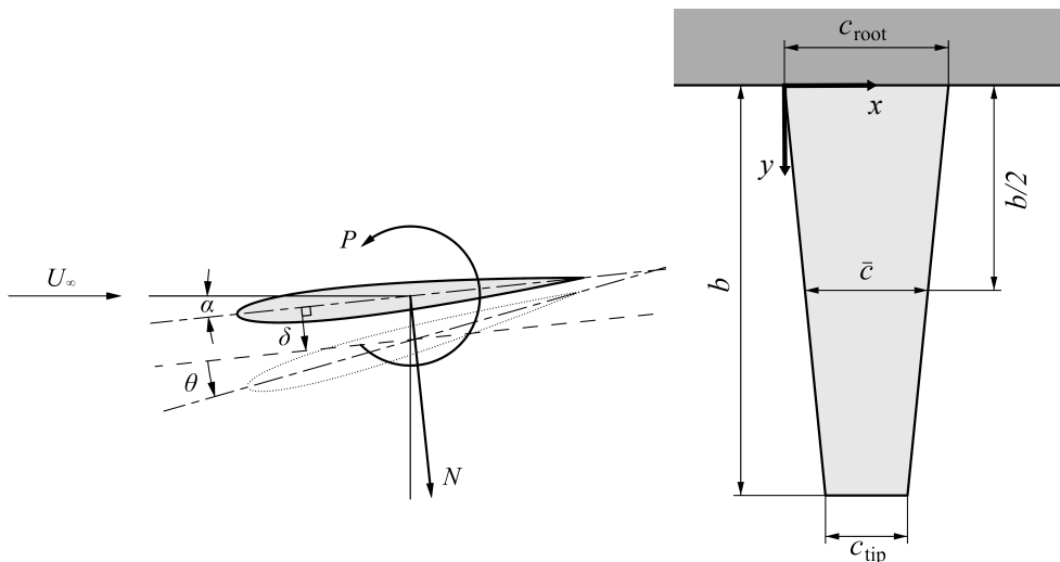
FIGURE 5. The coordinate system used for both the forces and tip deflection of the hydrofoil (left) is located at the mid-chord along the centreline. The deformed hydrofoil tip is represented by the dotted outline where the tip bending displacement, \delta , is measured by taking the mean displacement of the profile edge perpendicular to the centreline at the zero-load case. The tip twist deflection, \theta , is the rotation of the profile centreline from the zero-load case. A schematic of the hydrofoil's tapered planform (right) shows the coordinate system used in the analysis of the cavitation behaviour (e.g. cavity length) is located at the leading edge of the hydrofoil root.
