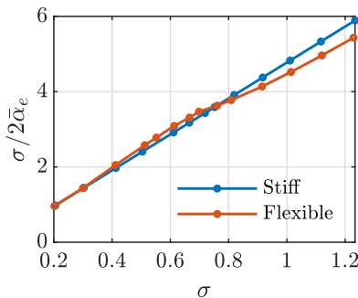
FIGURE 10. Comparing the cavitation parameter \sigma/2\bar{\alpha}_e of each hydrofoil for the \sigma range tested reveals the influence of \theta deformations on the cavitation behaviour. The flexible hydrofoil’s nose-up deformations for \sigma \geq 0.8 result in a decreased \sigma/2\bar{\alpha}_e value, suggesting accelerated cavitation regime transition for decreasing \sigma . The opposite occurs for 0.4 \leq \sigma \leq 0.75 with negative \theta increasing \sigma/2\bar{\alpha}_e , suggesting delayed regime transition.
