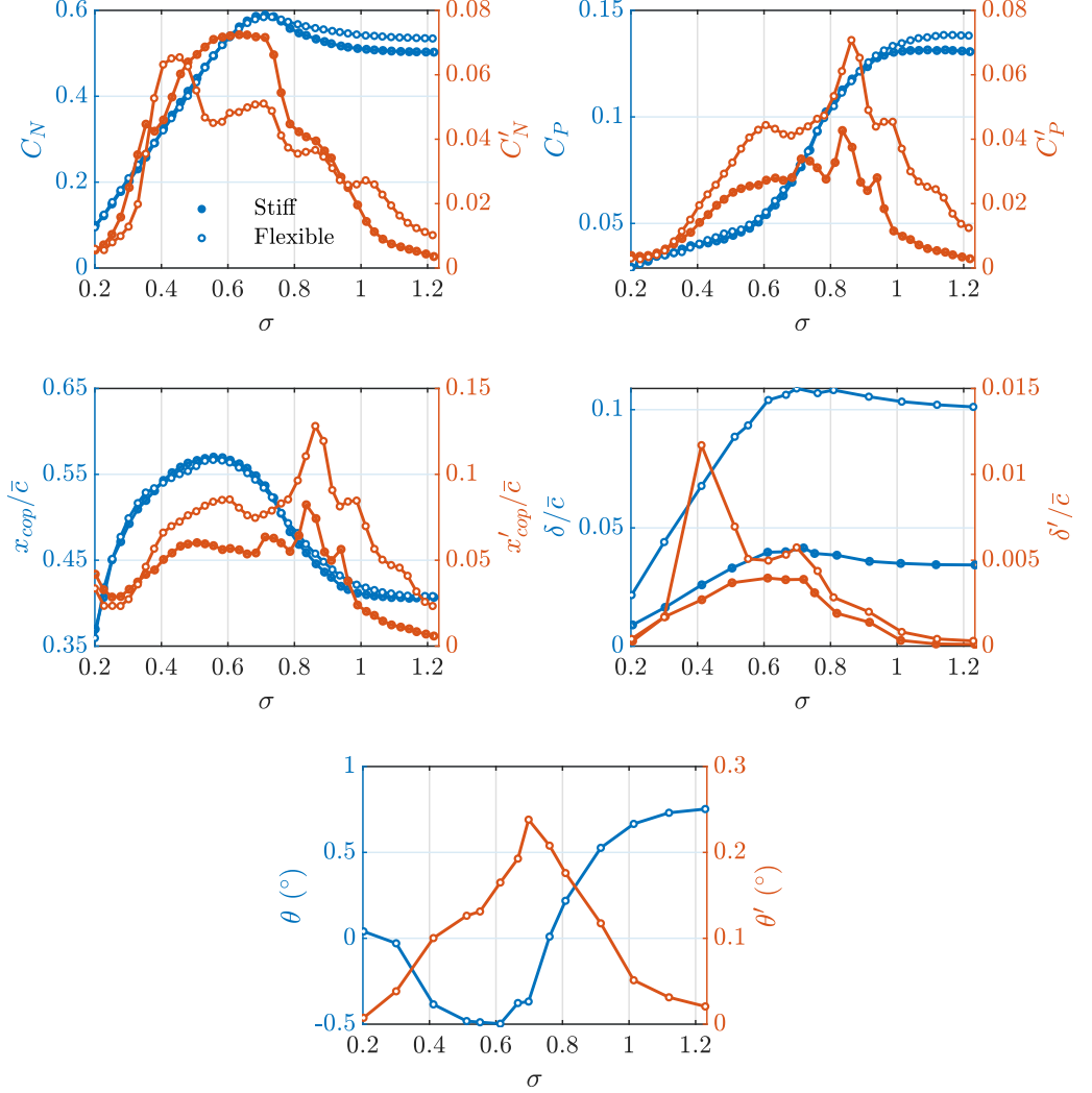
FIGURE 9. Mean and standard deviation values of the non-dimensional forces and deflections experienced by the stiff and flexible hydrofoils at various \sigma where ' indicates the standard deviation of the time varying quantity. The results show similar behaviour between the hydrofoils in the mean values of the normal force ( C_N ), pitching moment ( C_P ) and location of the centre of pressure ( x_{cop}/\bar{c} ) for varying \sigma . However, the degree of unsteadiness in the forces varies significantly between hydrofoils as indicated by the standard deviation. Tip displacement ( \delta/\bar{c} ) is much larger on the flexible hydrofoil for all \sigma with the twist angle ( \theta ) shifting from positive to negative based on x_{cop}/\bar{c} relative to the hydrofoils elastic axis.
