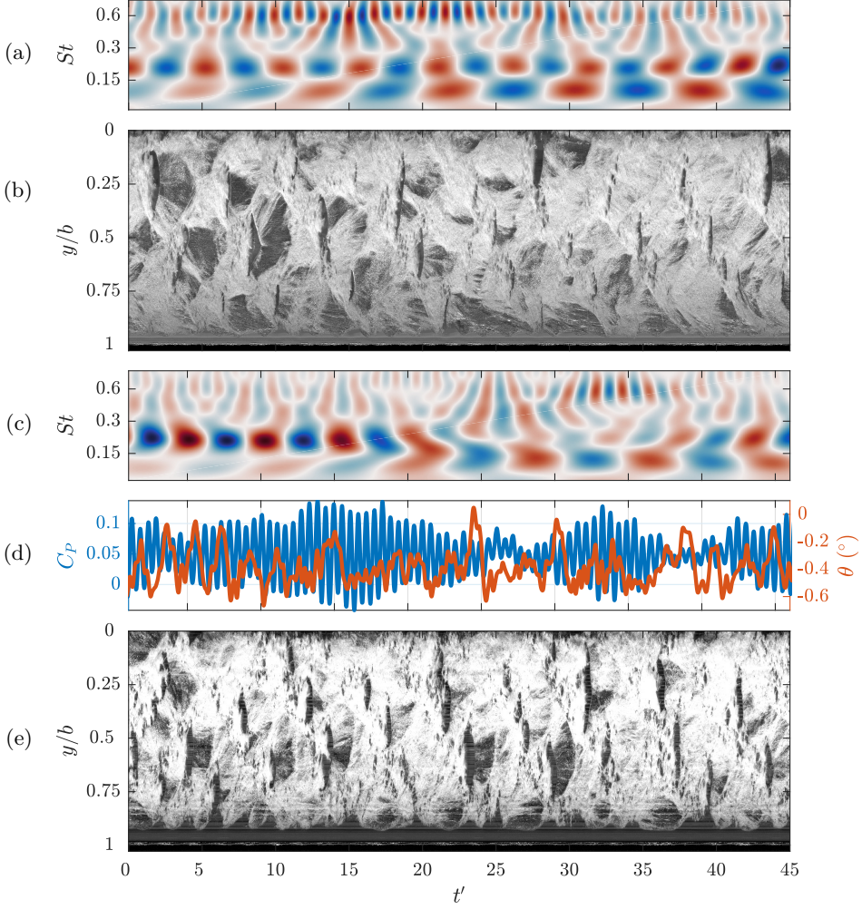
FIGURE 23. With several shedding mechanisms and modes active on each hydrofoil at a certain \sigma , the interactions and role of FSI becomes complex. At \sigma = 0.5 on the stiff hydrofoil, the C_N wavelet (a) shows the Type I ( St = 0.11 ) and IIa ( St = 0.19 ) modes being simultaneously active. Power of the Type I mode can be seen growing with t' in the C_N wavelet (a), corresponding with a change in the cavity physics evident in the spanwise space-time (b) taken at x/c_{\text{root}} = 0.58 . This multi modal behaviour is also observed on the flexible hydrofoil at \sigma = 0.55 where a clear transition in the C_N wavelet (c) is evident from the Type II mode ( St = 0.20 ) to the Type I mode ( St = 0.11 ) at t' = 20 . This transition is also evident in the \theta deformations (d) with oscillations shifting from high to low, as well as in the cavity dynamics where the spanwise space-time plot (e) at x/c_{\text{root}} = 0.65 shows larger cavitation clouds being shed along the span when the Type I mode is active.
