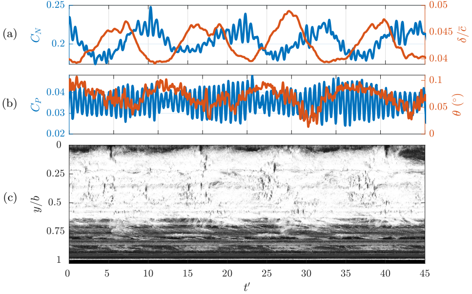
FIGURE 27. At \sigma = 0.3 , the phase lag between C_N and \delta/\bar{c} observed for the flexible hydrofoil at \sigma = 0.4 is still evident (a) with the \theta deformations (b) showing to be in phase with C_P at the Type I St = 0.10 frequency. The weakening of the shockwave-driven shedding as the flexible hydrofoil approaches the transition to supercavitation is evident in the spanwise space-time plot (c) taken at x/c_{\text{root}} = 0.73 showing minimal cavity break-up.
