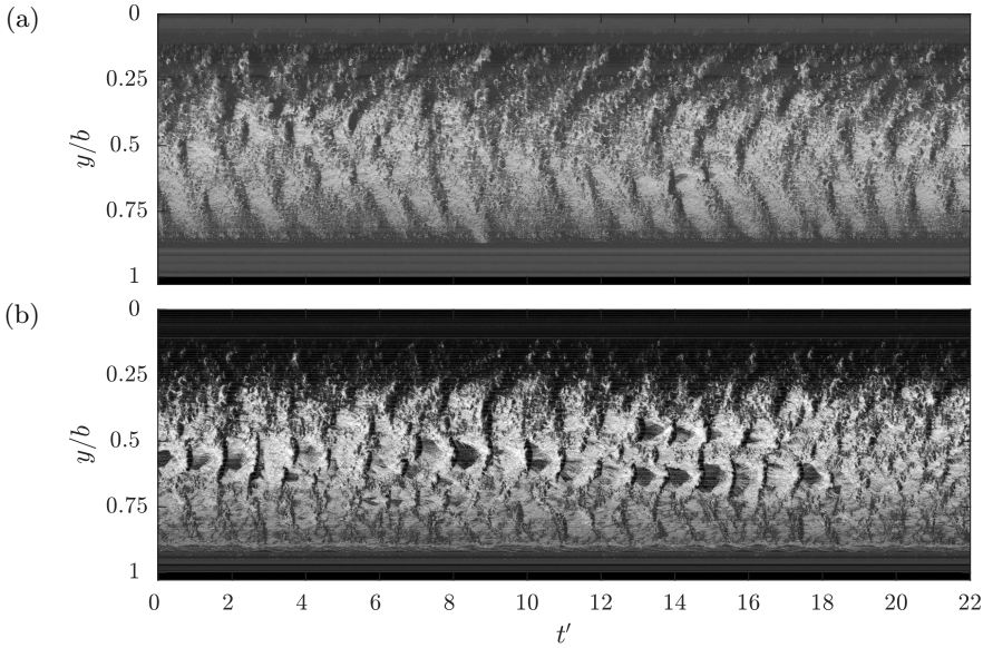
FIGURE 18. Spanwise space-time plots representing sheet cavitation just prior to a regime transition with reducing \sigma of the stiff hydrofoil (a) taken at x/c_{\text{root}} = 0.35 and \sigma = 1.1 as well as the flexible hydrofoil (b) taken at x/c_{\text{root}} = 0.31 and \sigma = 1.2 . Where the stiff hydrofoil is seen to experience cavity break-up solely driven by interfacial instabilities, the flexible hydrofoil shows intermittent manifestations of re-entrant jet formation as it is closer to cloud cavitation transition.
