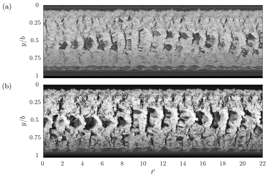
FIGURE 19. Spanwise space-time plots showing cloud cavitation of the stiff (a) and flexible (b) hydrofoil taken at x/c_{\text{root}} = 0.31 and x/c_{\text{root}} = 0.35 , respectively, for and \sigma = 1.0 . The re-entrant jet remains confined to around mid-span due to three-dimensional effects on each hydrofoil. The stiff hydrofoil exhibits a slightly higher shedding frequency of St = 0.74 compared to St = 0.61 on the flexible which is linked to induced \theta angle increasing \sigma/2\bar{\alpha}_e and cavity length.
