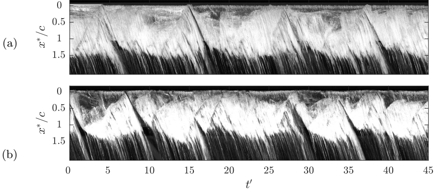
FIGURE 26. Chordwise space-time plots of the stiff (a) and flexible (b) hydrofoil both taken at y/b = 0.25 for \sigma = 0.3 and 0.4 , respectively, showing the cavity dynamics for solely Type I shockwave-driven shedding. Both hydrofoils exhibit the growth, stable and shockwave phases for each cycle, however the flexible hydrofoil exhibits more inconsistent cycles in terms of cavity dynamics and cycle duration.
