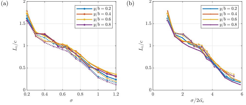
FIGURE 8. Attached cavity length, L_c , against \sigma (a) and \sigma/2\bar{\alpha}_e (b) with cavity length taken at the point of cavity break-off for various positions along the span for the stiff (.....) and flexible (—) hydrofoils. The cavity length is non-dimensionalized by the local chord, c , at each of the spanwise positions, showing continuous cavity growth as \sigma is reduced.
