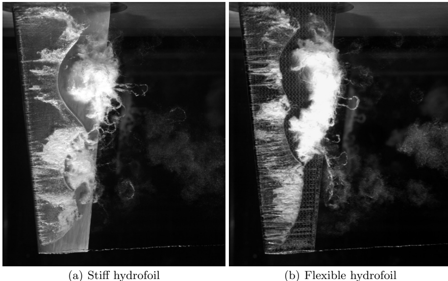
FIGURE 1. Cloud cavitation about a finite span hydrofoil exhibiting multiple shedding events along the span due to the re-entrant jet instability and spanwise compatibility of the cavitation. The hydrofoil is vertically mounted at an incidence of 6^\circ to the flow with a chord-based Reynolds number, Re = 0.8 \times 10^6 and \sigma = 0.7 .
