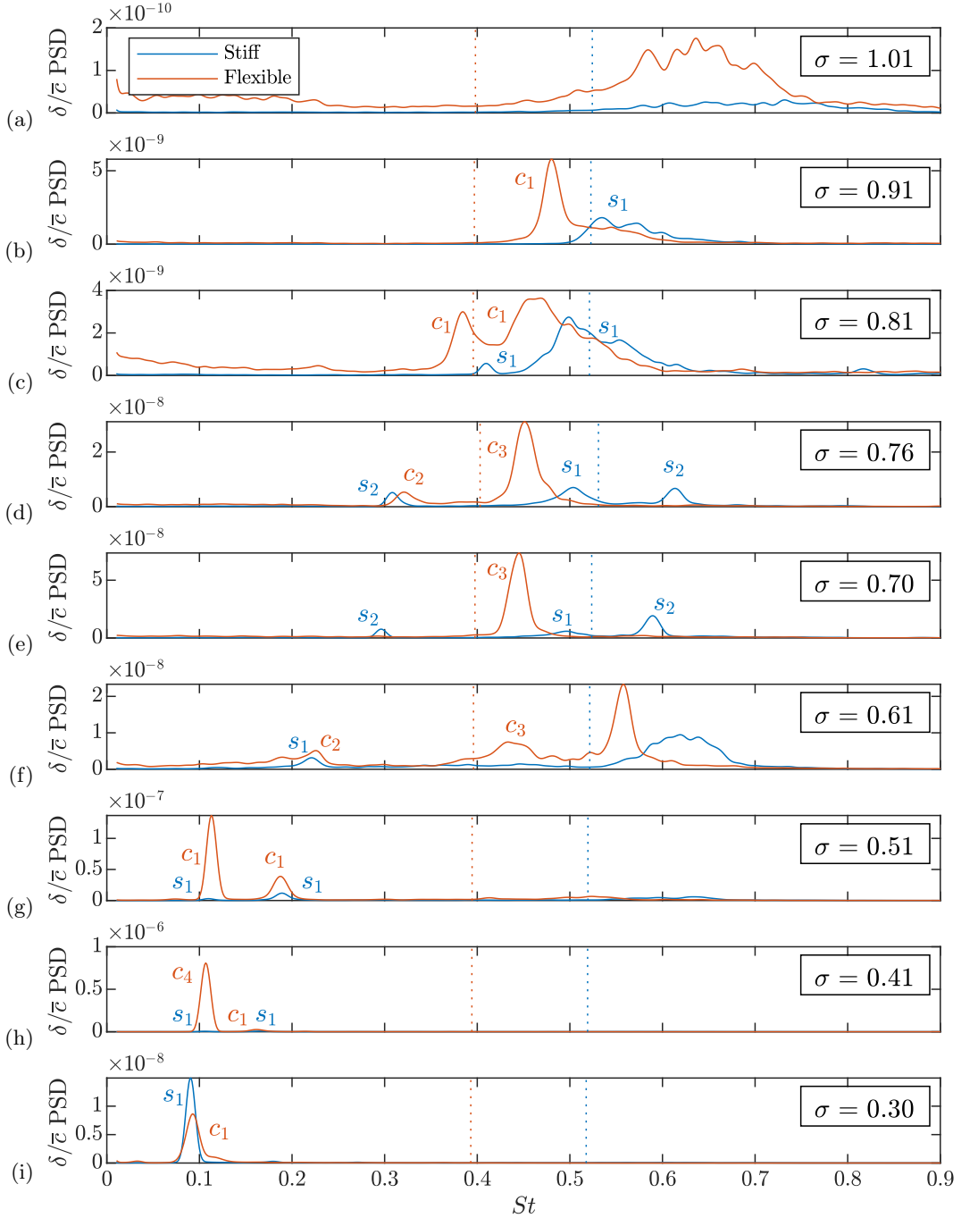
FIGURE 16. \delta/\bar{c} PSD for both the stiff and flexible hydrofoils at key values of \sigma with the modes annotated using the labels from table 4. The spectra show the shedding modes modulates as \sigma varies. Lock-in of the shedding events with either the natural frequency (dashed lines) or the harmonics of the hydrofoils is evident, particularly on the flexible hydrofoil at St = 0.44 and 0.11 for \sigma = 0.7 and 0.4 , respectively, due to its lower stiffness. Note the change in the order of magnitude between each plot.
