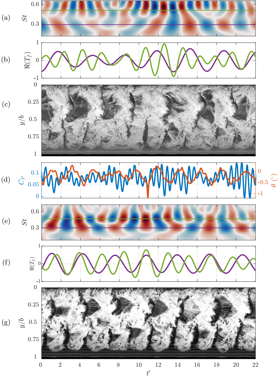
FIGURE 21. The multi-modal behaviour on either hydrofoil is shown in plots of the real values of Morlet wavelet transforms for C_N (a(stiff), e(flexible)) at \sigma = 0.7 . Extracting the Type IIa and IIb wavelet components at St = 0.29 and 0.49 for the stiff hydrofoil (b) and St = 0.30 and 0.44 for the flexible hydrofoil (f), respectively, shows the correlation with shedding events. This shedding events along the span are evident in the spanwise space-time plots taken at x/c_{\text{root}} = 0.5 and 0.58 for the stiff (c) and flexible (g) hydrofoils, respectively.
