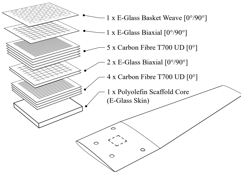
FIGURE 3. Lay-up sequence of the flexible composite hydrofoil.
