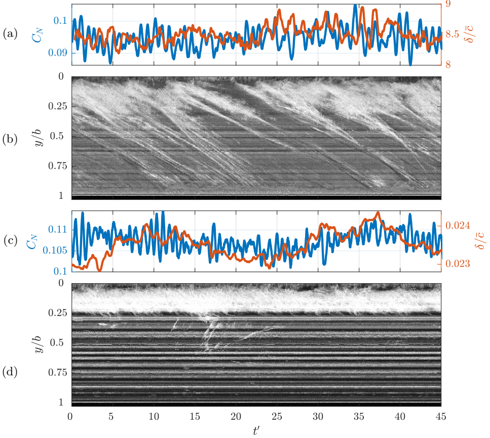
FIGURE 28. Synchronised time series of the normal force ( C_N ) and tip displacement ( \delta/\bar{c} ) at \sigma = 0.2 for the stiff (a) and flexible (c) hydrofoil. The spanwise space-time plots of the stiff (b) and flexible (d) taken at x/c_{\text{root}} = 0.75 show minimal activity in the supercavity as it closes far enough downstream to prevent shedding mechanisms from forming.
