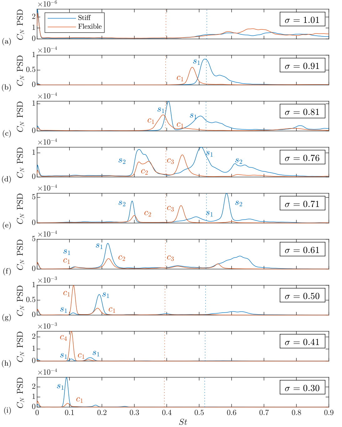
FIGURE 15. C_N PSD for both the stiff and flexible hydrofoils at key values of \sigma with the modes annotated using the labels from table 4. The spectra show the shedding modes shift in frequency as \sigma varies. The lock-in phenomena is evident in both hydrofoils with large amplification of C_N at \sigma = 0.7 and 0.4 . Lock-in occurs when the excitation frequency from the shedding matches either the natural frequency (dashed lines) itself, or one of its harmonics. Note the change in the order of magnitude between each plot.
